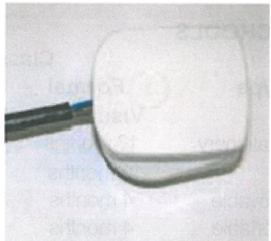
3b Inadequate strain relief
